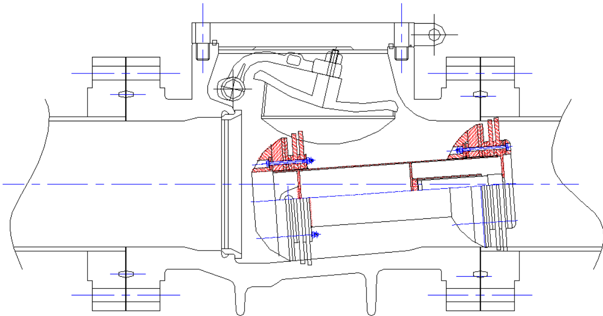
(Figure.1. 20"ns Uni-Di pig traversing check valve in reverse)
